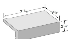
Modular Edge Cap 2 1/4" x 3 5/8" x 7 5/8"
