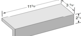
Norman Edge Cap 3 5/8" x 2 1/4" x 11 5/8"
