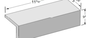
Utility Edge Cap 3 5/8" x 3 5/8" x 11 5/8"
